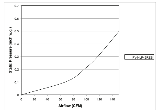
Resistance Curve 4" or 6" duct
