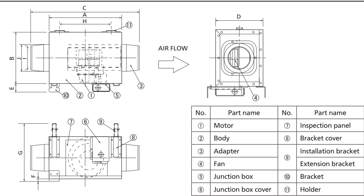
Dimensions: mm(inch)
